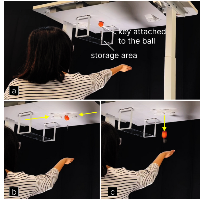
Figure 16: Ceiling Storage Application – (a) Users can attach items, such as a key, to the thrown object and store them to the ceiling by throwing. The wheeled robots will (b) push out the items to a location that is right above the users' hand and (c) drop them to the users.
