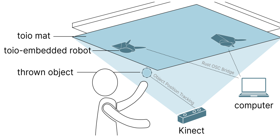
Figure 3: Our implementation of ThrowIO includes an overhanging ferromagnetic toio mat, two toio-embedded robots controlled wirelessly by a central computer, and a thrown object whose location is tracked by a Microsoft Kinect v1 camera placed underneath the toio mat.
