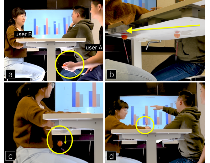
Figure 18: In-Person Communication Application – (a) A person is passing a pen under the table while hoping not to distract the presenter. (b) The wheeled robots push and (c) drop the pen to another person (d) so she could use the pen.
