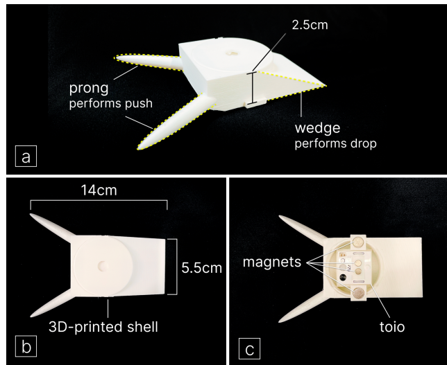
Figure 4: The robot is designed to perform (a) push and drop operations, enabled by (b) a 3D-printed shell mounted on (c) a toio robot.
