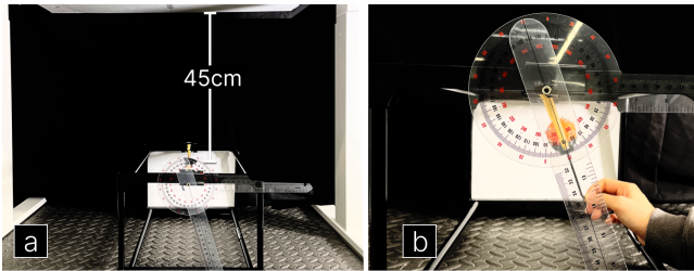
Figure 9: (a) In our evaluation setup where a slingshot mechanism was implemented, (b) we pulled the slingshot down at different angles and distances to vary the throwing speed.
