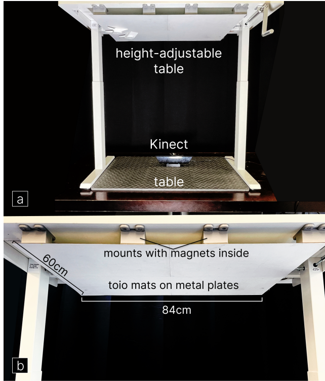
Figure 6: (a) In our setup, we put the height-adjustable table on top of a normal table where we place the Kinect camera. (b) The proposed height-adjustable overhanging surface is built by placing toio mats on a ferromagnetic metal plate that is overhung by custom magnetic 3D-printed structures.
